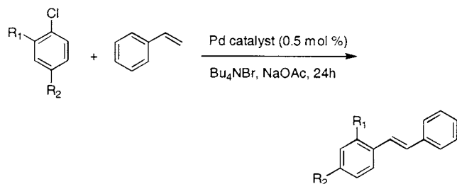
Scheme 1. Pd-Catalyzed Heck Reaction of Aryl Chlorides with Styrene
